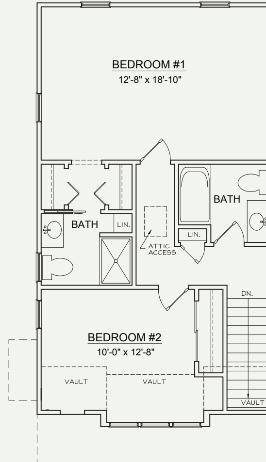
Second Floor 633 square feet
